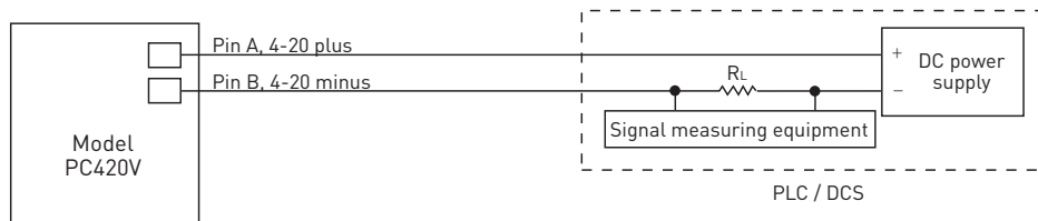
Typical circuit
