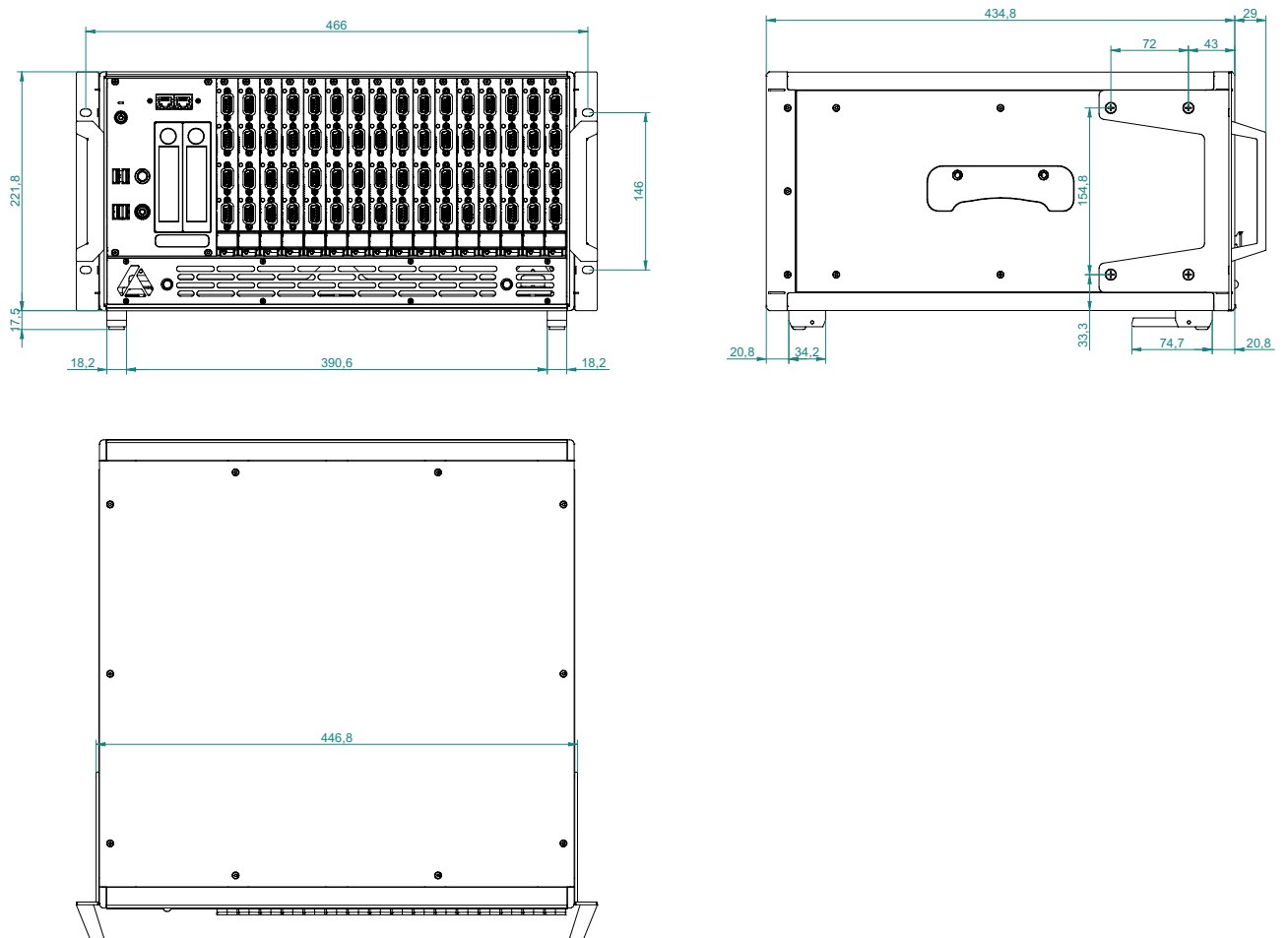
Fig. 1: Dimensions DEWE3-RMx / DEWE3-PA8-RM
