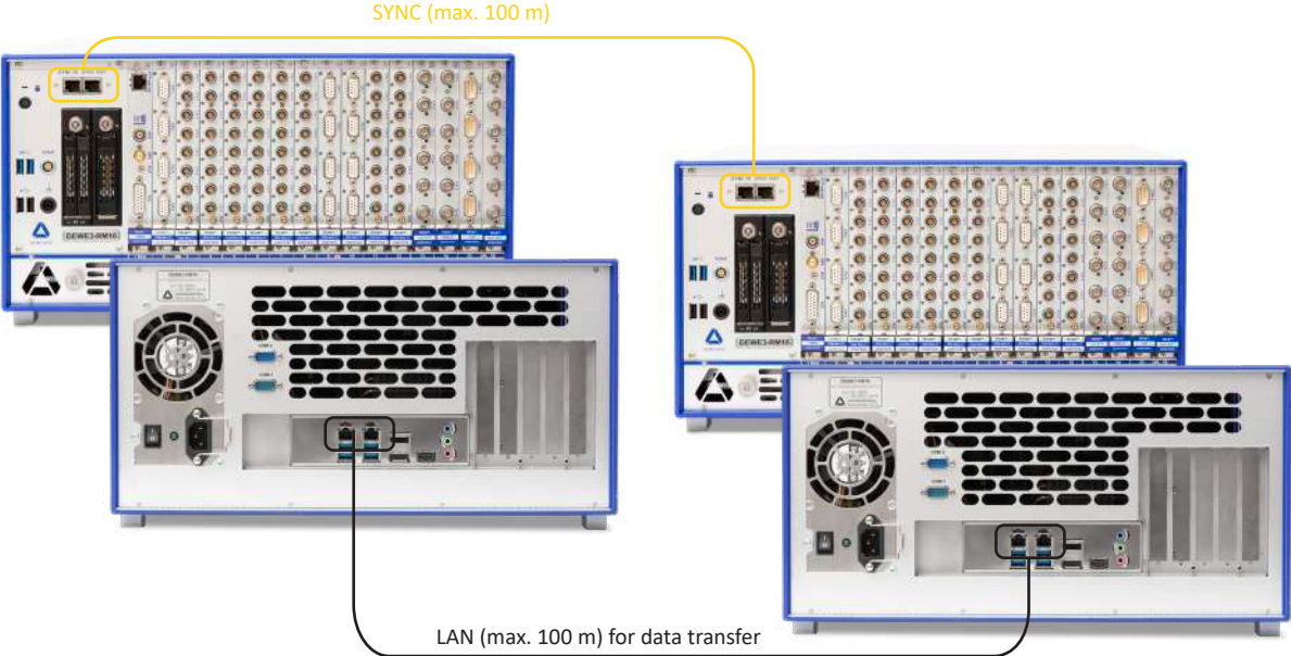
Fig. 24: Network with multiple systems
