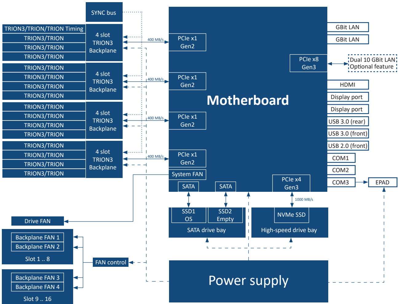
Fig. 2: Block diagram
