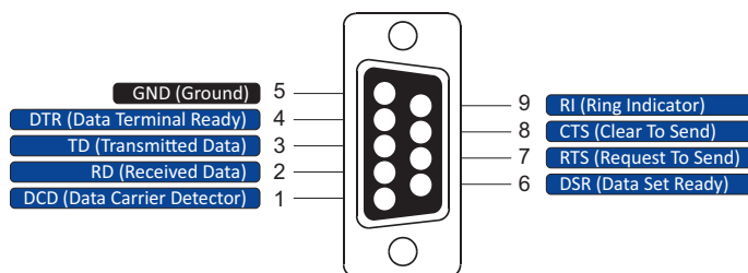
Fig. 5: Pin assignment RS-232 interface connector (COM 1+2)
