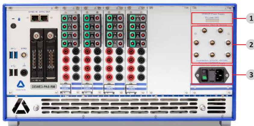
Fig. 6: Additional ports for DEWE3-PA8-RM
