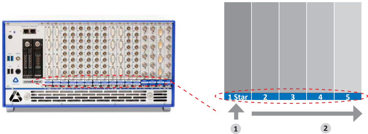
Fig. 8: STAR-slot for TRION timing/sync modules
