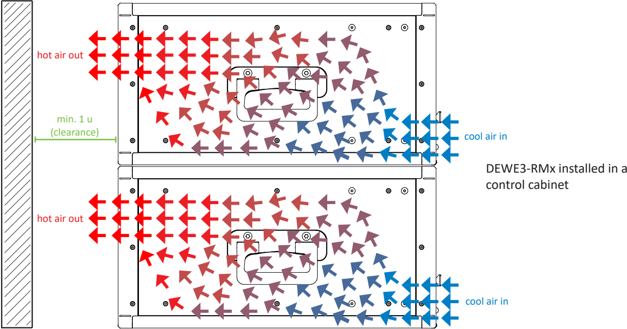
Fig. 12: Cooling concept for control cabinet use
