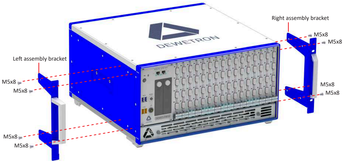
Fig. 10: Installing the 19" mounting brackets
