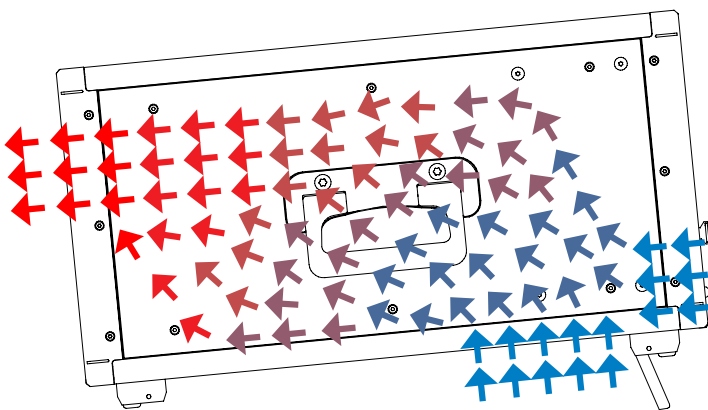
Fig. 11: Cooling concept for benchtop instrument use
