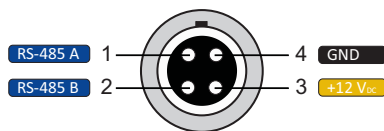
Fig. 4: Pin assignment EPAD2 connector
