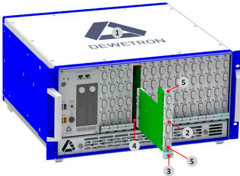
Fig. 7: Installing a TRION module
