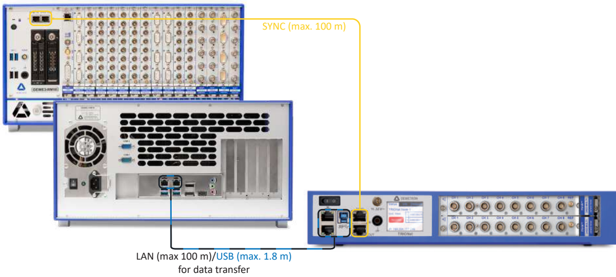
Fig. 23: Channel expansion with TRIONet
