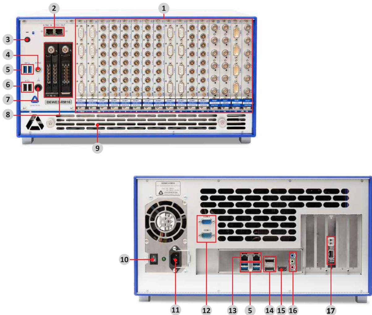
Fig. 3: Connections and ports DEWE3-RMx / DEWE3-PA8-RM
